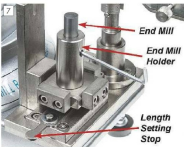
Using the depth setting jig.
